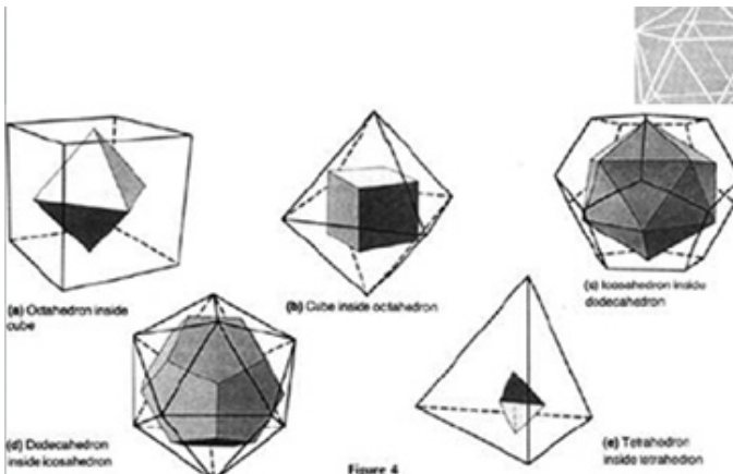
Figure 4 THE PLATONIC DUALS
