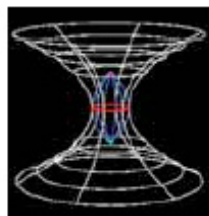
Schwarzschild geometry
