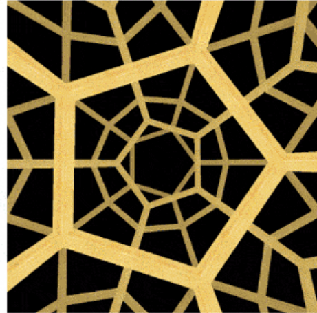
An image showing the view in a dodecahedral space universe (Image credit: Jeff Weeks)
