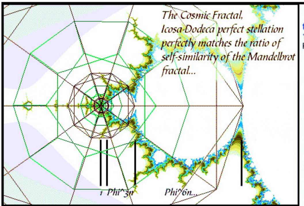
Exponents of GOLDEN RATIO Defining the Mandelbrot Fractal (and DNA's top view)
